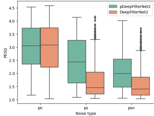
Fig. 2: Box plot featuring the PESQ for DeepFilterNet2 and pDeepFilterNet2 (unified encoder version) for different noise types: primary speaker + noise (pn), primary speaker + secondary speaker (ps), primary speaker + secondary speaker + noise (psn).
