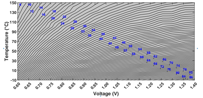
(a) AFN at 7 years, stress: V_{dd}=1.2V and Temp.=100^\circ C .
