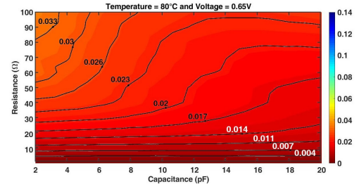
(a) V_{dd}=0.65V
