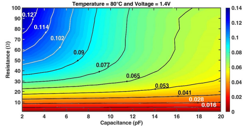
(c) V_{dd}=1.4V
