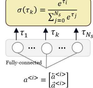
Fig. 2: The schematic of the attention unit.
