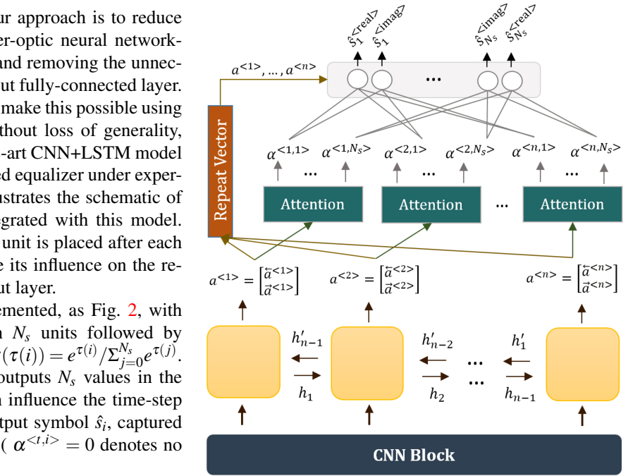
Fig. 1: The schematic of the attention-integrated CNN+RNN model. The CNN block initially processes the input to capture short-temporal dependencies. The output feature map is then passed to a recurrent layer to capture long-term features. There exists one attention unit on top of each RNN time-step.
