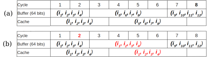
Figure 11. Hypothesis of Replay of four instruction as the cache is enabled, (a) normal execution process, (b) replay of four instruction caused by LFI-induced 64-bit buffer update prevention during clock cycle 2.
