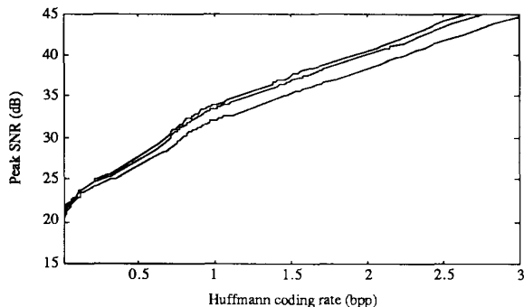
Figure 7: PSNR vs. Huffman bit rate for a “non-Daubechies” filter ( L = 12 , K = 2 ), designed with transition bandwidths \Delta\omega = 0.0625 , 0.1 , and 0.14 . PSNR is globally higher for increasing values of \Delta\omega .
