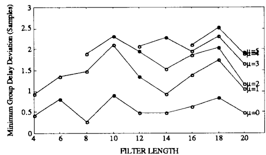
Figure 3: Minimum group delay deviation (in the pass-band) of “closest to linear phase” filters H(z) versus lengths L for several values of \mu = L/4 - K/2 . Solutions closest to linear phase are obtained for \mu = 0 (Daubechies filters [3]).
