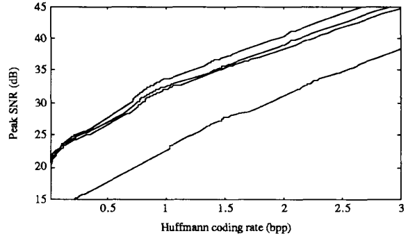
Figure 5: PSNR vs. Huffman bit rate for 4 filters of length L = 12 and transition bandwidth \Delta\omega = 0.0625 , corresponding to K = 0, 2, 4 , and 6 (PSNR increases as K increases). Optimization was made using bit rate after Huffman coding as coding criteria.
