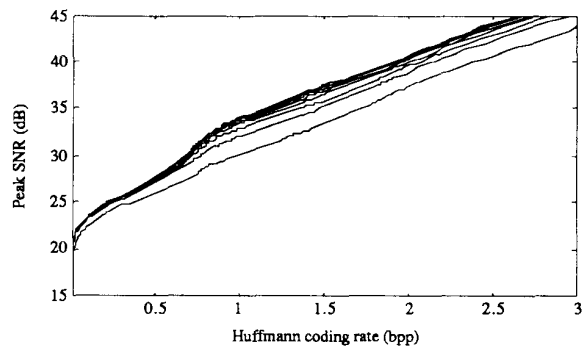
Figure 6: PSNR vs. Huffman bit rate for Daubechies filters of different lengths ( L ranging from 2 to 18). PSNR first increases as length increases, until an asymptote is reached (for L \approx 12 ). Performance is not improving for longer filters (PSNR curves are even lowered a bit).
