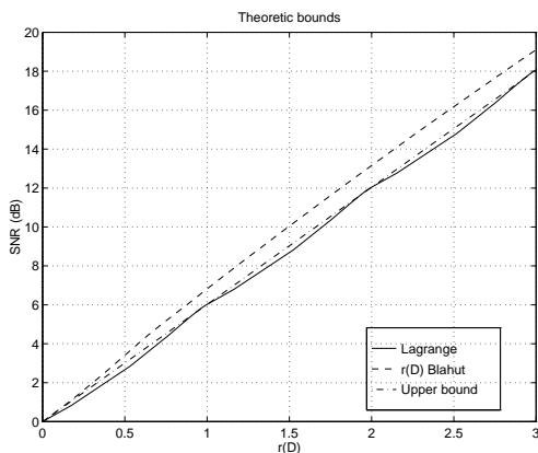
Figure 6: Solid: Theoretical OPTA curves (Lagrange, Blahut) and the upper bound for p = 0 .
