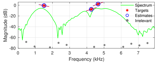
Figure 3: NLR resolved close frequency components, even though they were obfuscated under the same local maximum (peak) in the magnitude spectrum.
