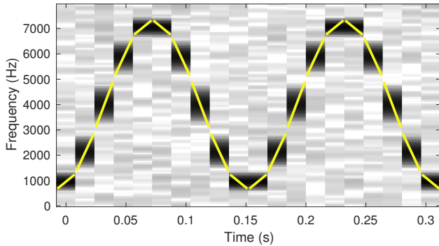
(a) Fast chirp rate estimation from a noisy cosine FM sound.
