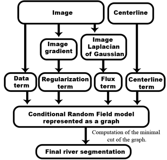
FIGURE 12. Flowchart describing the third step of the algorithm that uses the previously computed centerline along with the SAR image to detect the river.
