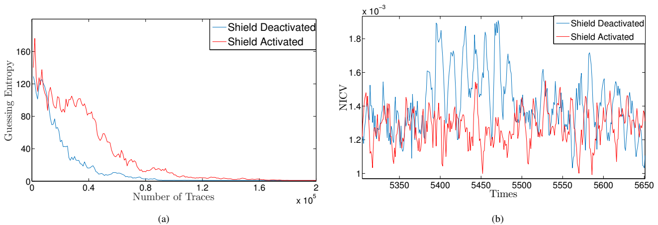
Fig. 13. (a) Guessing Entropy computation for AES with activated/deactivate shield. (b) NICV computation for AES with activated/deactivate shield.
