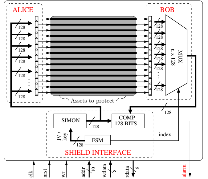
Fig. 2. Cryptographically secure shield structure
