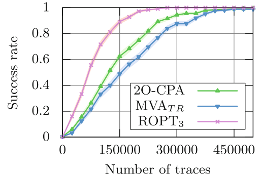
(f) \sigma = 9
