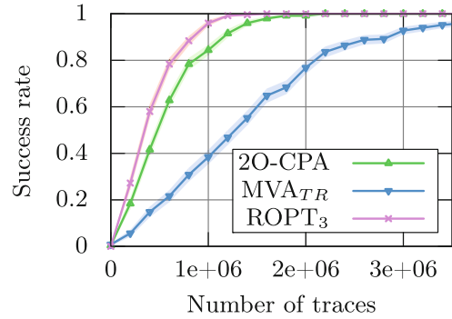
(h) \sigma = 13
