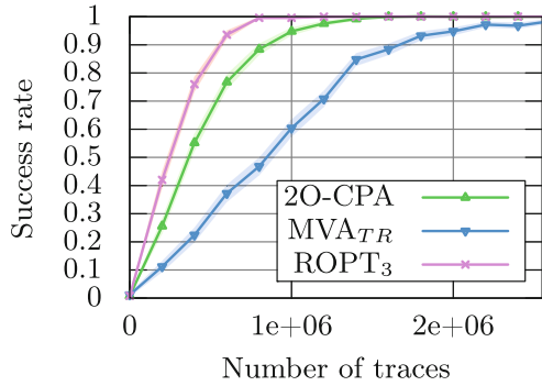
(g) \sigma = 12
