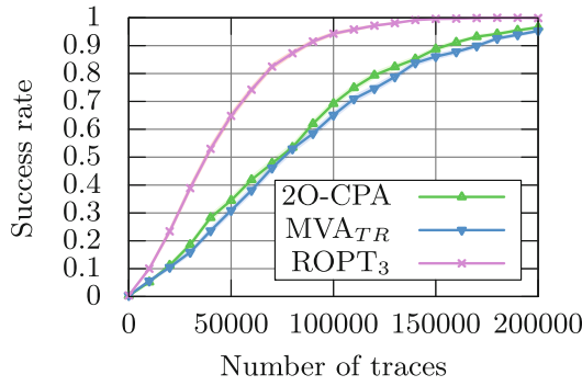
(e) \sigma = 8
