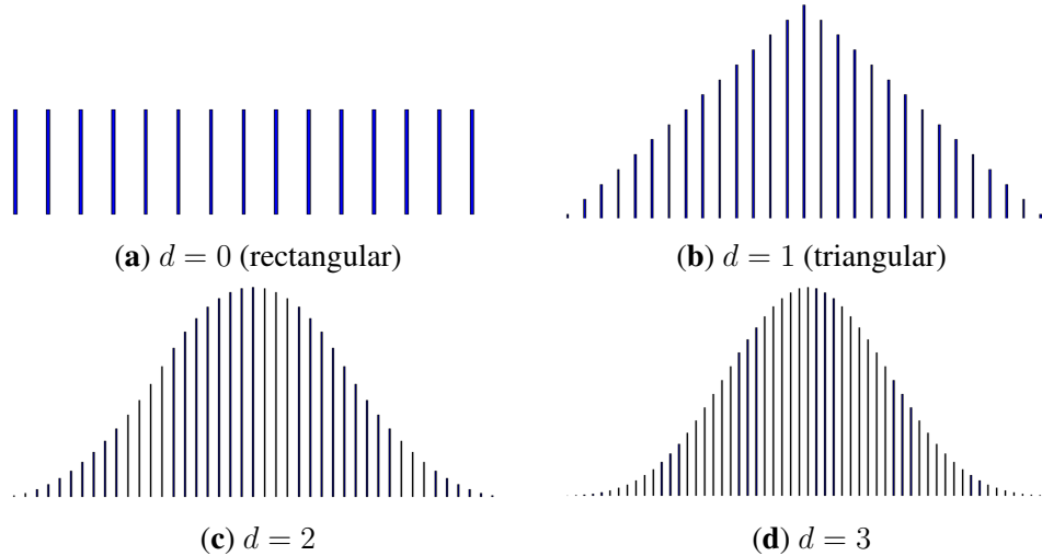
Figure 1. Discrete plots of input probability distributions (of X_d ) that attain capacity for M = 15 and different values of d .
