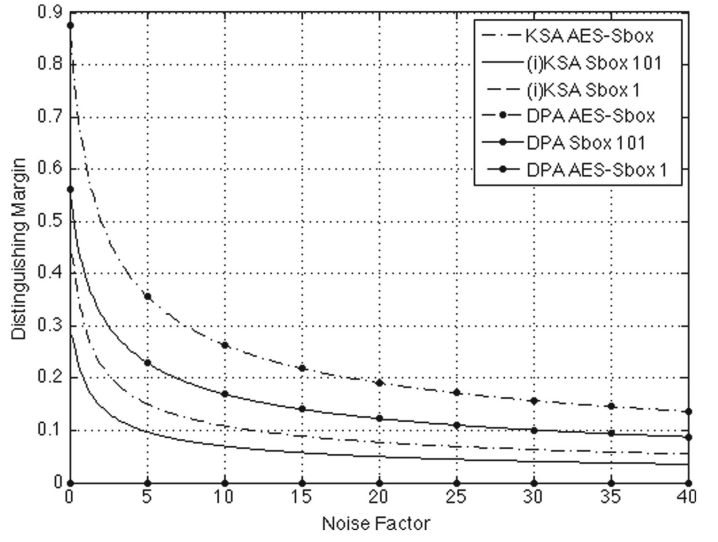
Fig. 5. Distinguishing margin for the studied S-boxes.
