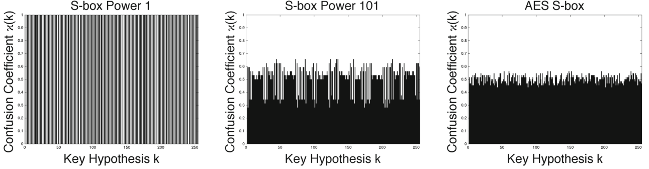
Fig. 4. Confusion coefficients for S_1 , S_{101} and S_{254}
