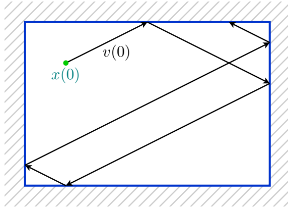
Figure 1: Example of ray trajectory in the classical rectangular billiard. The discrete directional measure \sigma assigns the same weight to the four directions taken by the ray trajectory, including \mathbf{v}(0) . The trajectory is interrupted after six reflections to avoid overloading the figure, but after that it will explore space uniformly over time.
