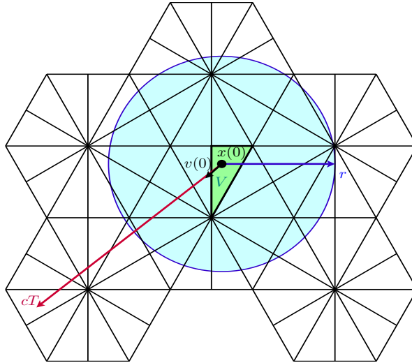
Figure 2: Strict space tessellation by the hemiequilateral triangle. The original polygon V is painted green, and its reflections V_j are left empty. The original position \mathbf{x}(0) [resp. direction \mathbf{v}(0) ] of the ray trajectory is represented by the small black disk (resp. small black arrow). The meanings of the blue disk and blue arrow, as well as the red arrow, are explained in Remark 6.
