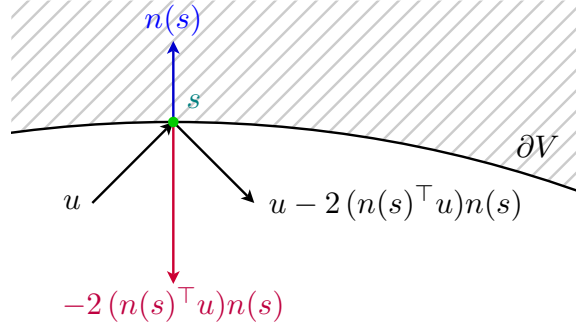
Figure A.3: Specular reflection of the incident vector \mathbf{u} at \mathbf{s} \in \partial V , where \mathbf{n}(\mathbf{s}) is the outward normal to the boundary \partial V at point \mathbf{s} .
