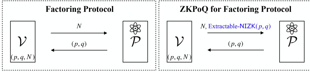
Figure 3: Diagram of ZKPoQ for factoring-based scheme.
