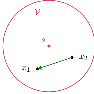
Figure 1: Interior points: the two space positions \mathbf{x}_1 and \mathbf{x}_2 belong to the same vicinity \mathcal{V} \subset V (red circle) of an interior point \mathbf{s} \in V , so that the direct path from \mathbf{x}_2 to \mathbf{x}_1 (green arrow) is included in \mathcal{V} .
