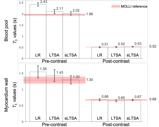
Fig. 3. T_1 values from the mid-ventricular slice in the intracavitary blood pool and myocardium. Horizontal lines correspond to the MOLLI reference. Error bars indicate the standard deviation in the region.
