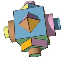
GlobFit [LWC*11]
