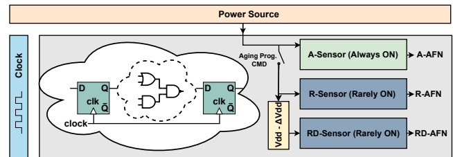
Figure 9: Our proposed sensor setup for aging prognosis.
