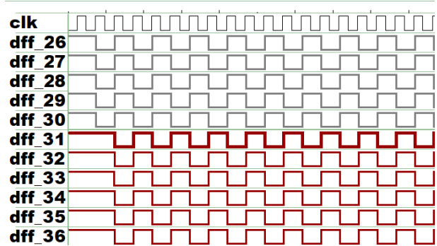
Figure 6: Waveforms of Fig. 5 in (V, T) = (1.2V, 27°C), where n_0 = 9 and n_1 = 43 .
