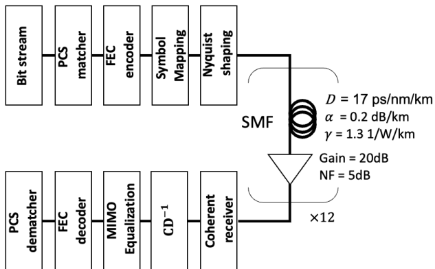
Fig. 4. Transmission chain
