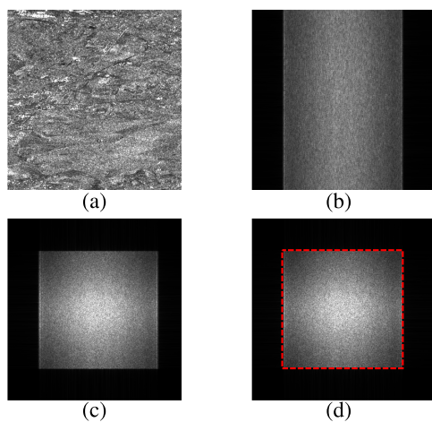
Figure 7 Effect of deramping and demodulation on a TOPS Sentinel-1 SLC product. (a) the amplitude of the SLC image; (b) the complex Fourier spectrum; (c) the deramped spectrum; (d) the deramped and demodulated spectrum
