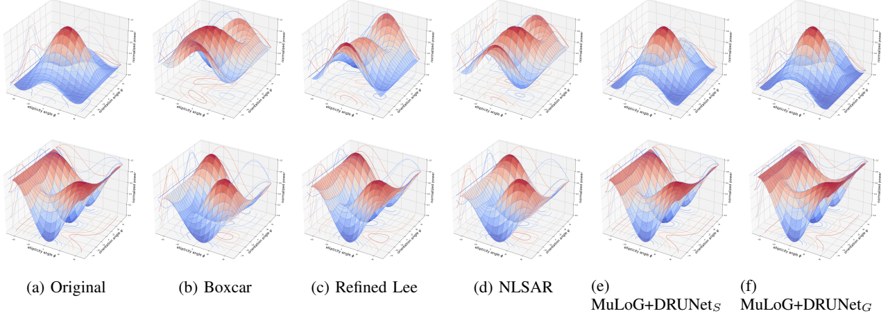
Figure 6: Co-pol (first row) and cross-pol (second) computed from the average covariance matrix of the 3 \times 3 area of the first image in figure 5 mark by a green box.
