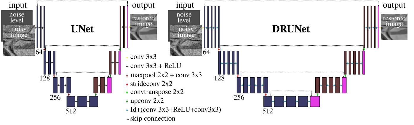
Figure 2: Comparison of UNet and DRUNet architectures.
