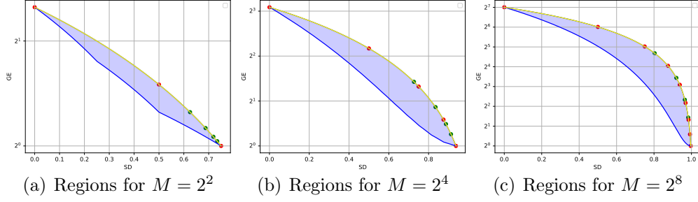
Figure 3: Regions G(K|Y) vs. \Delta(K|Y) as given by Theorem 11. The 4 green dots are the exact values computed for Q = 1, 2, 3 , and 4 traces for deterministic Hamming weight model. The red dots corresponds to subset of bits revealed. The yellow curve corresponds to the formula G = \frac{M+1}{2} - \frac{M\Delta}{2} and is a one-to-one relationship for deterministic leakage models and uniform secret.
