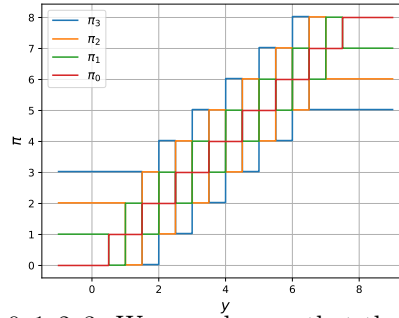
Figure A.11: \pi_i(y) for i = 0, 1, 2, 3 . We can observe that the \pi_i are step functions. Their are constant on the interval of the form [\frac{p}{2}, \frac{p+1}{2}) for all integer p .
