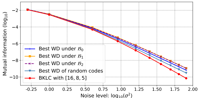
Fig. 7 Information-theoretic evaluation of the best weight distributions (WD) under different bases as shown in Table 4.
