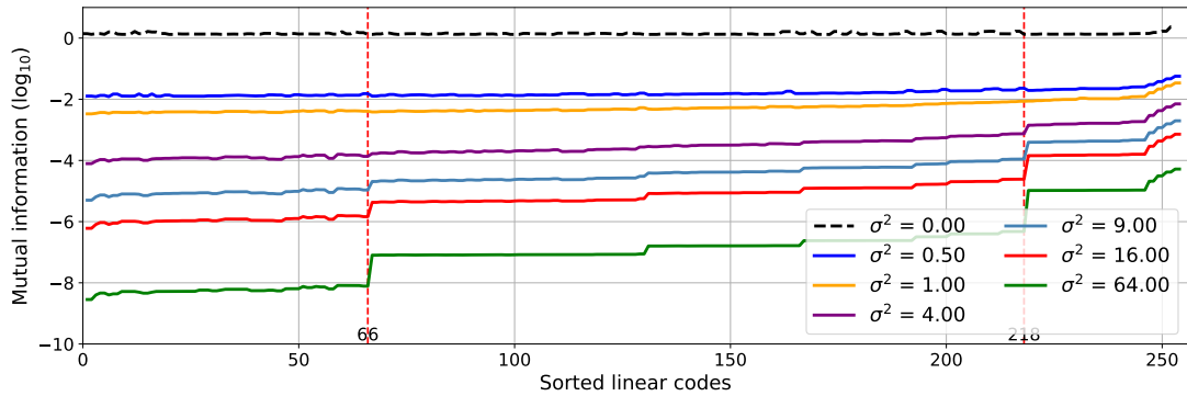
Fig. 6 Information-theoretic evaluation of all 254 candidates under the default basis \mathcal{B}_2 sorted in the lexicographical order.
