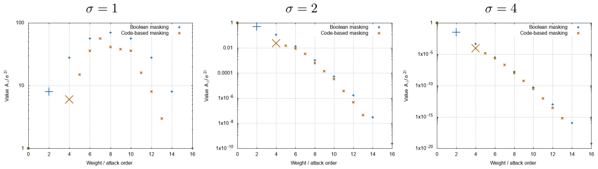
Fig. 3 Value of A_i/\sigma^{2i} per weight (or equivalently, per attack order). Largest symbol indicates leading term.
