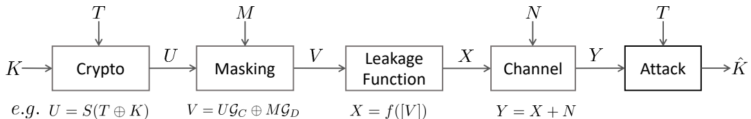
Fig. 1 Side-channel leakage setup and subsequent analysis modelization (modified from [11]).
