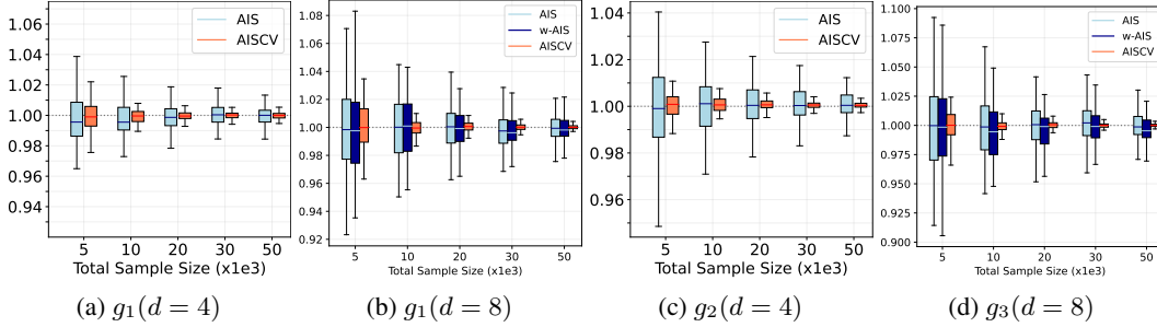
Figure 4: Integration on [0, 1]^d : boxplots of estimates I_n^{(ais)}(g) and I_n^{(aiscv)}(g) with integrands g_1, g_2, g_3 in dimensions d \in \{4; 8\} obtained over 100 replications. The true integral equals 1.
