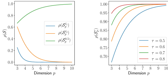
Figure 3. Evolution of the Ratio Volume with dimension p .
