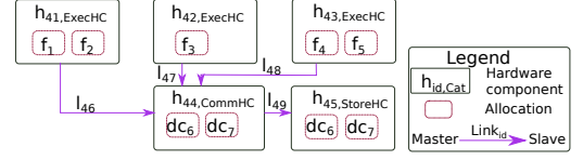
Fig. 3 Graphical representation of an allocation model
