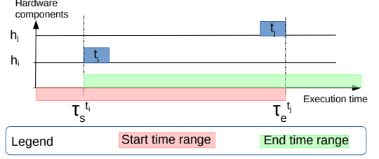
Fig. 5 Illustration of the cross function
