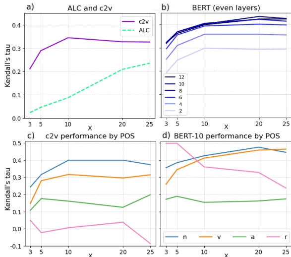
Figure 2: a and b : Kendall’s tau obtained by different vector representations on SemCor. We only include even layers for BERT for better readability. c and d : Performance of c2v and BERT (10th layer) by PoS.
