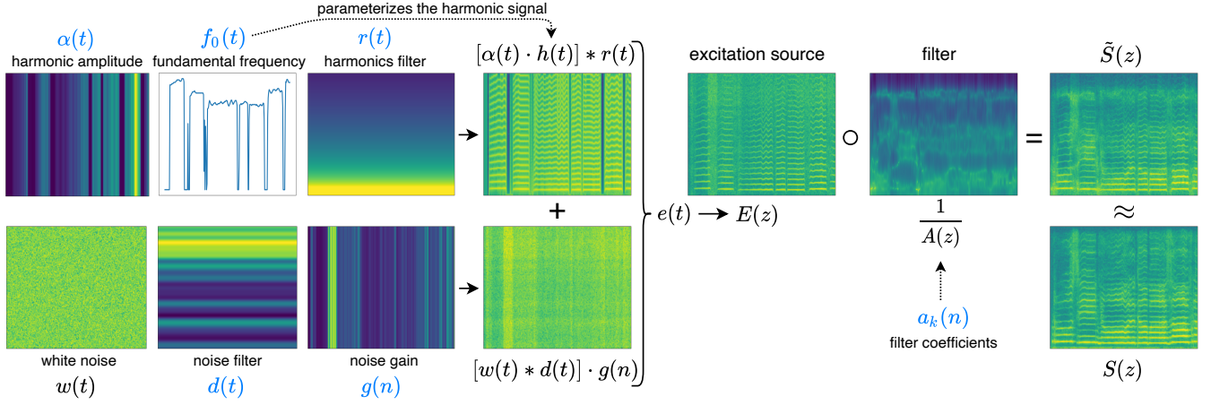
Fig. 2. Exemplary overview of the source-filter model decomposition. The model parameters are denoted in blue font. The ‘ \circ ’ denotes element-wise multiplication. Although most components are visualized through magnitude spectrograms, processing is not necessarily done in the time-frequency domain.
