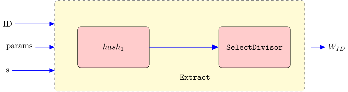
Figure 1: Extract algorithm
