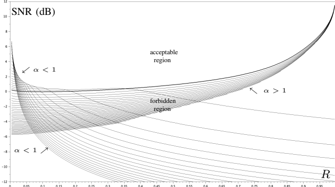
Fig. 6. Lower bounds on SNR vs. coding rate for n = 1024 on a BSEC. The thick curve is for \alpha = 1 .
