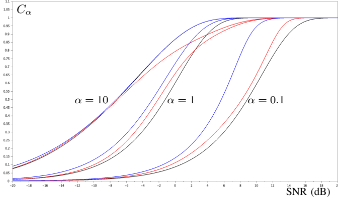
Fig. 3. \alpha -capacities of binary-input BSC (black), BSEC (red) and AWGN channel (blue) as a function of SNR = 1/(2\sigma^2) per transmitted bit.
