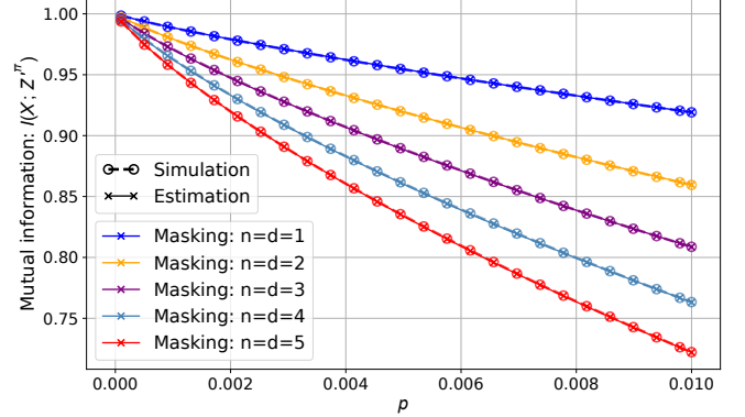
Fig. 3. Numerical evaluation and theoretical estimation of mutual information I(X; Z^n) for n \in \{1, 2, 3, 4, 5\} under weak noise. Note that d = w_H(\Pi) is the number of attacker's probes and the estimation is calculated by Theorem 6.
