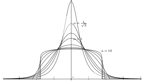
Fig. 1. \alpha -Gaussian distributions (154) for \alpha = 3^{-3/4}, 3^{-1/2}, 3^{-1/4}, 1, 2, 4, 8, 16 .
