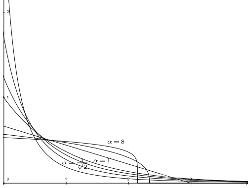
Fig. 2. \alpha -exponential distributions (156) for \alpha = 2^{-3/4}, 2^{-1/2}, 2^{-1/4}, 1, 2, 4, 8 .
