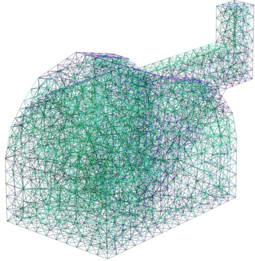
Figure 5: Resulting nonuniform tetrahedral mesh.
