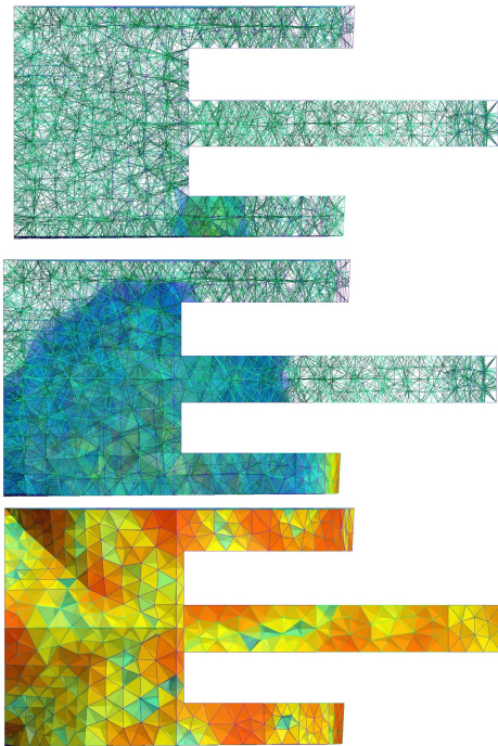
Figure 8: Time evolution of simulated pressure field from initial impulse to diffuse field, view from above the cave. Top: after 1ms; middle: after 8ms; bottom: after 1.5s.
