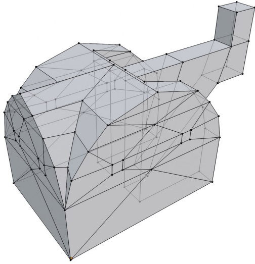
Figure 4: Wireframe of the cave geometry.
