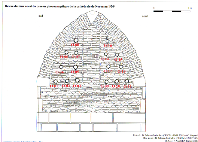
Figure 2: An example of an accurate mapping of one of the phonicamptic cave walls with the acoustical pots' positions.
