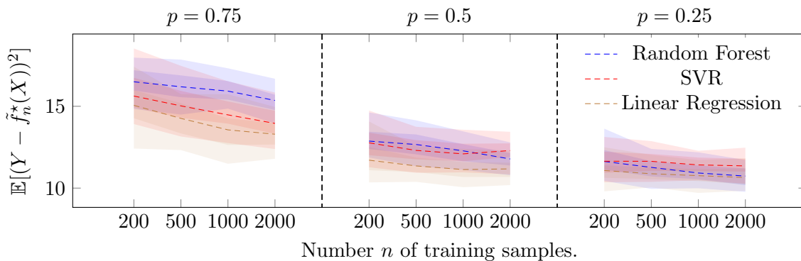
Figure 8: Prediction error \mathbb{E}[(Y - \tilde{f}_n^*(X))^2] for the three predictive models (SVR, random forest and linear regression) using the IPCW LoO for data generated by the Cox model (16).
