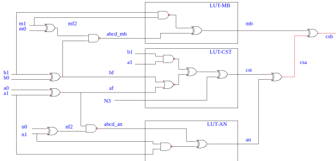
Fig. 2: Masked circuit computing csb_1 . The leaking signals (red color) are csa_1 and csb_1 .
