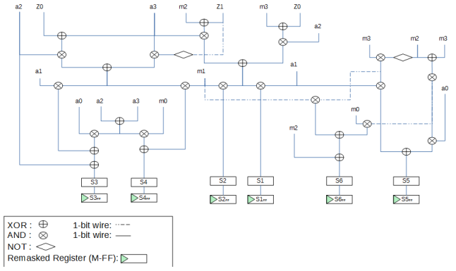
Fig. 3: Our new design of one bit GF_{2^4} inversion - Formally proven to resist against glitches.
