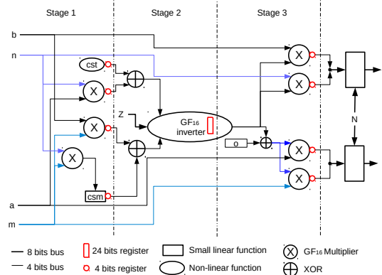
Fig. 10: AES S-Box scheme using our secure GF_{24} inverter.
