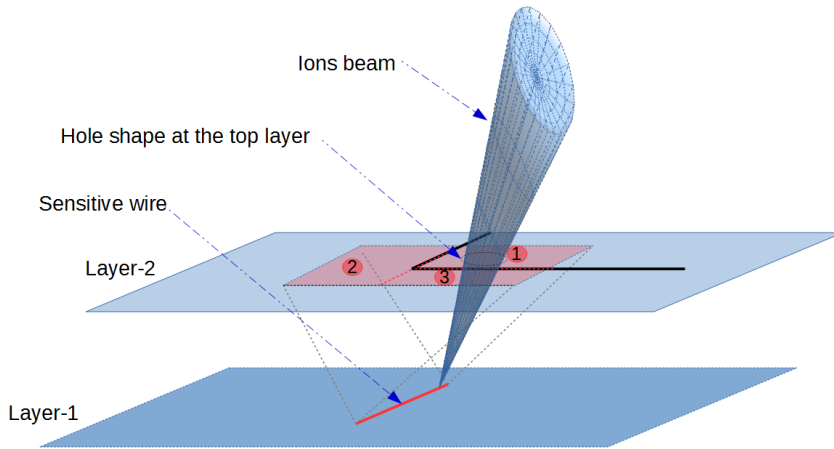
Fig. 5: Illustration of the FIB model for milling.
