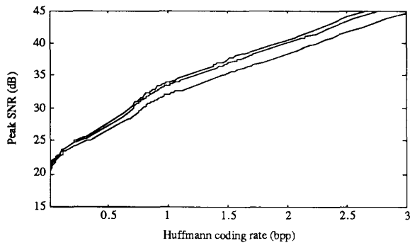
Figure 7: PSNR vs. Huffman bit rate for a “non-Daubechies” filter ( L = 12 , K = 2 ), designed with transition bandwidths \Delta\omega = 0.0625 , 0.1 , and 0.14 . PSNR is globally higher for increasing values of \Delta\omega .
