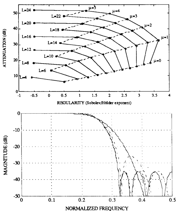
Figure 2: (a). Attenuation (in dB) vs. "Sobolev" regularity [7] for the families of filters obtained. (b). Obtained low-pass filters frequency responses |H(e^{j\omega})|^2 with (normalized) transition bandwidth \Delta\omega = 0.14 and length L = 16 . Daubechies and Smith-Barnwell filters (solid) correspond to K = 8 and 0 , respectively. Intermediate filters are shown for K = 2 (dashed), K = 4 (dotted) and K = 6 (dash-dotted).
