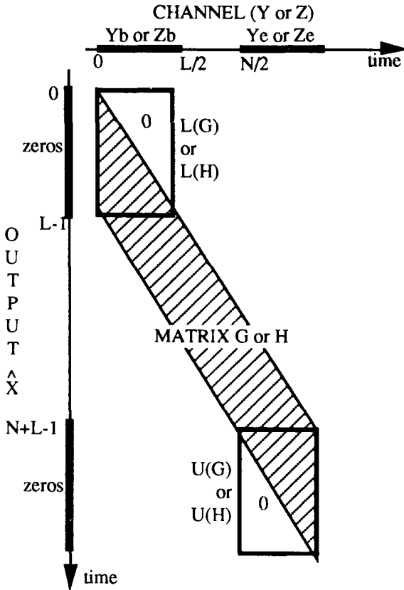
Figure 2. Schematic matrix description of the synthesis bank, meant to represent the formula \hat{X} = \mathbf{G}Y + \mathbf{H}Z , where \mathbf{G} and \mathbf{H} are interpolation+convolution matrices corresponding to the synthesis filters.
