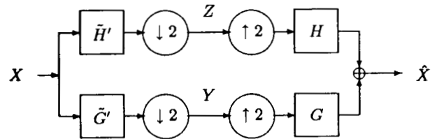
Figure 1. A two-band perfect reconstruction FIR filter bank. All filters are assumed to be of even length L . The tilde symbol denotes time reversal: this convention on the analysis filters will simplify subsequent formulations. Output \hat{X} is equal to X delayed by L-1 samples.
