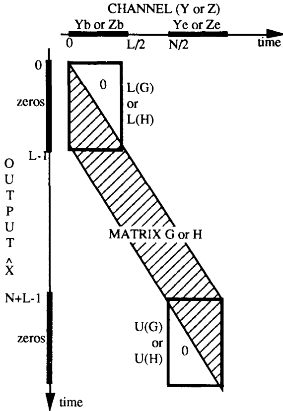
Figure 2. Schematic matrix description of the synthesis bank, meant to represent the formula \hat{X} = \mathbf{G}Y + \mathbf{H}Z , where \mathbf{G} and \mathbf{H} are interpolation+convolution matrices corresponding to the synthesis filters.
