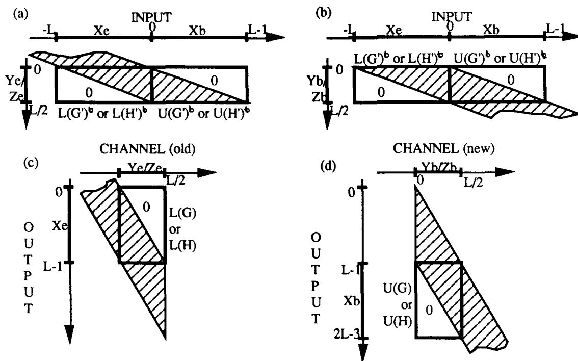
Figure 5. Schematic matrix description of the transition during analysis (a), (b) and synthesis (c), (d), for the "old" filter bank (a),(c) and the "new" one (b), (d).
