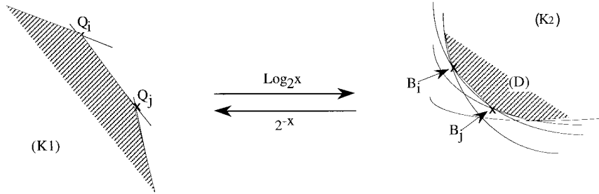
Fig. 7. Vertices in the equivalent constrained optimization problems. Each vertex ( Q_i ) of the feasible domain ( K1 ) is linked by the function x \mapsto \log_2 x to a virtual vertex ( B_i ) in ( K2 ). The virtual vertices of ( K2 ) are the vertices of the convex polyhedron ( D ).
