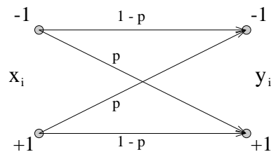
Figure 2: Binary symmetric channel model with \pm 1 outputs.
