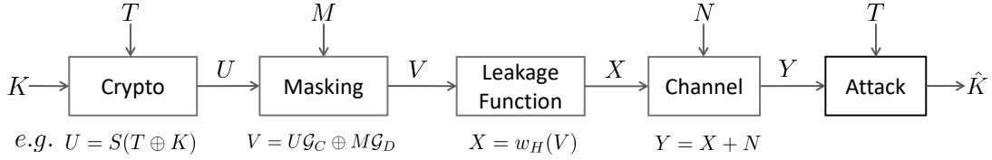
Figure 1: Side-channel leakage setup and subsequent analysis modelization (modified from [8]).
