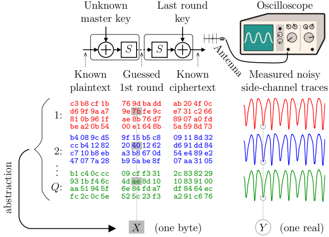
Fig. 1. Public information (plaintext and ciphertext) available to an attacker and first-round key-dependent intermediate (discrete) value, put in front of corresponding side-channel traces (analog) observed by the attacker.
