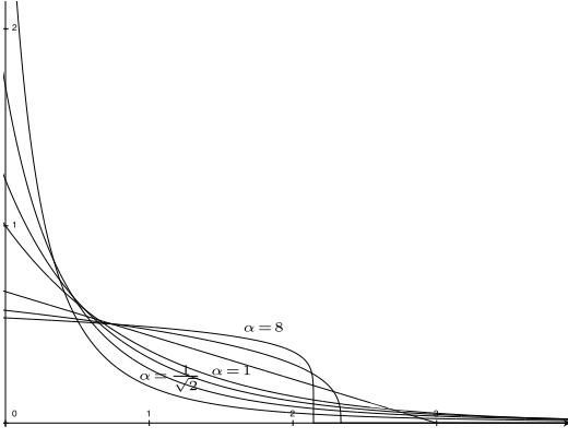
Fig. 2. \alpha -exponential distributions (156) for \alpha = 2^{-3/4}, 2^{-1/2}, 2^{-1/4}, 1, 2, 4, 8 .
