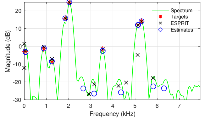
Figure 3: NLR resolved close frequency components, even though they were obfuscated under the same local maximum (peak) in the magnitude spectrum.
