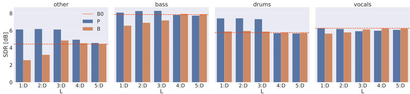
Figure 2: Median over all tracks of the median SDR (expressed in dB) over each track for different fine-tuning strategies and different instruments in the dataset. Blue bars correspond to models adapted with the proposed loss while Orange ones correspond to models adapted using a reconstruction loss only. The horizontal red line represents the B0 baseline, i.e. , the original ConvTasnet before adaptation.
