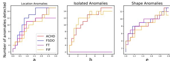
Figure 4: Number of anomalies detected over a grid of parameters for three types of anomalies (location, isolated, and shape) for ACHD and three further state-of-the-art methods.
