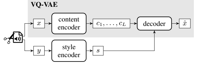
Fig. 1. A high-level depiction of the proposed method. We extract pairs of segments from audio files and use them for self-supervised learning of a VQ-VAE with an additional style encoder. The content representation c_1, \dots, c_L is discrete, the style representation s is continuous.
