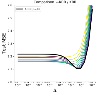
Figure 3. Test MSE w.r.t. \Lambda
