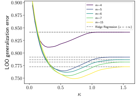
Figure 8. LOO error w.r.t. \kappa
