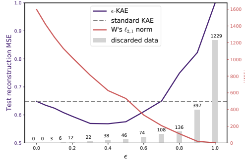
Figure 7. Reconstruction error w.r.t. \epsilon
